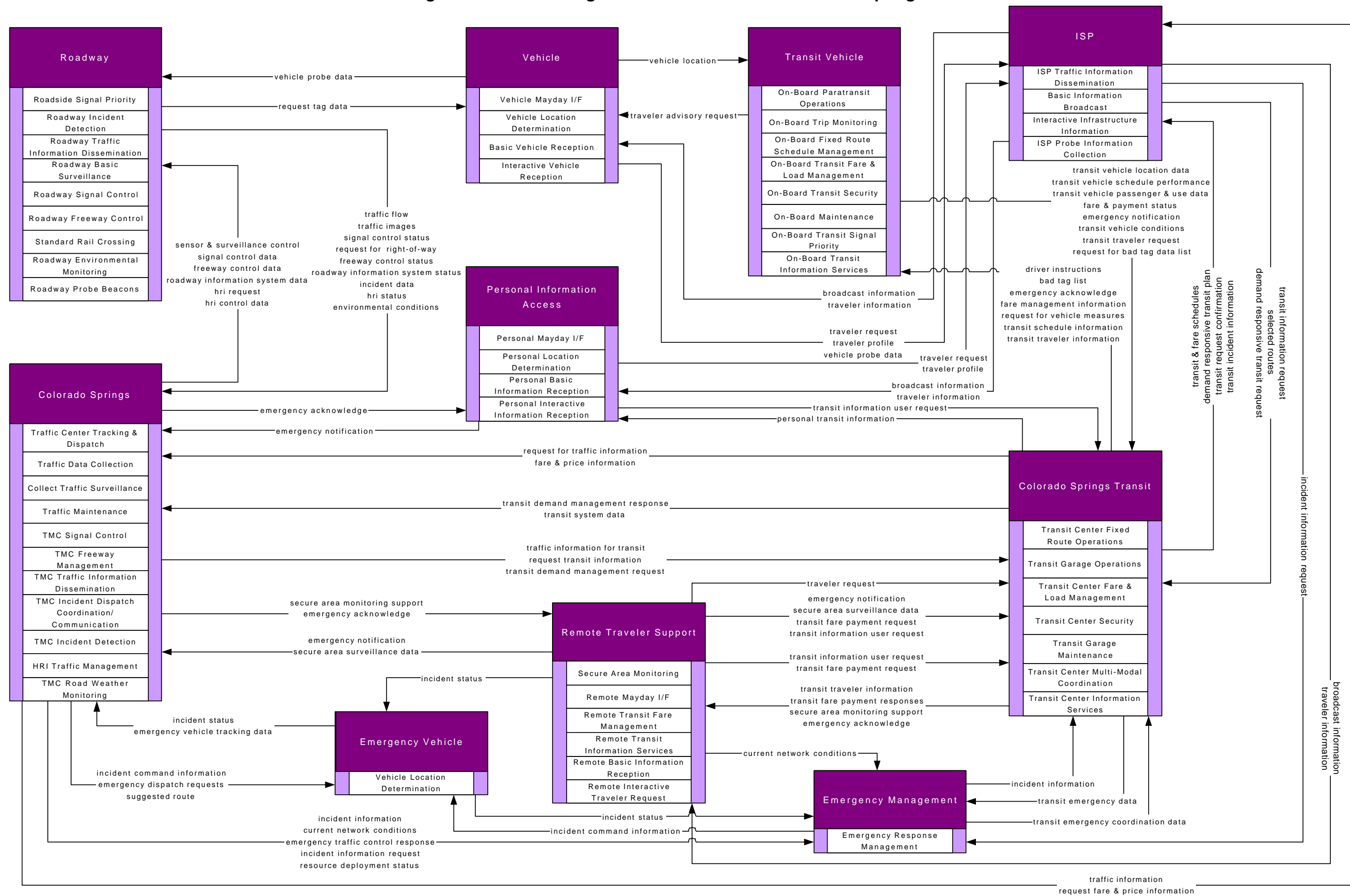
Figure A - 8: CDOT Region 2 ITS Architecture – Colorado Springs View
