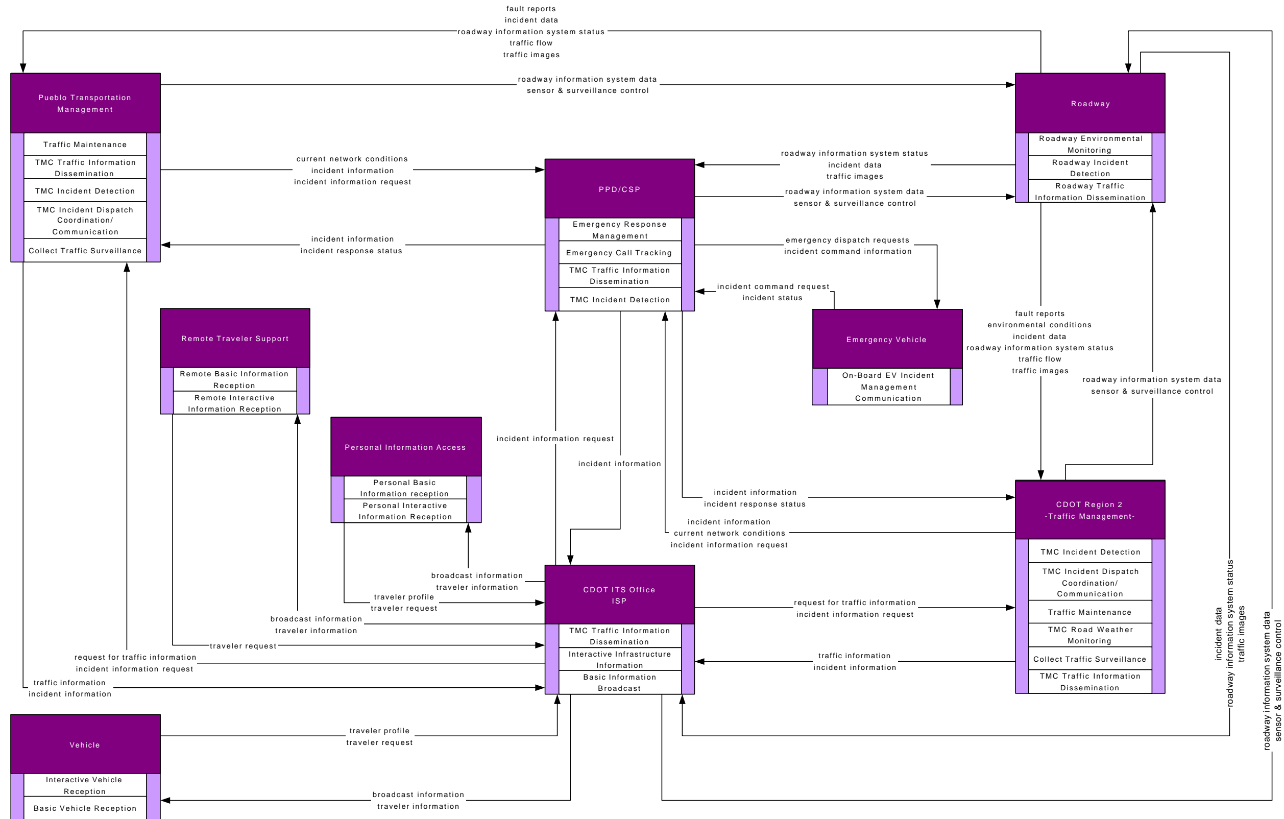
Figure A - 1: Pueblo FMS Project ITS Architecture
