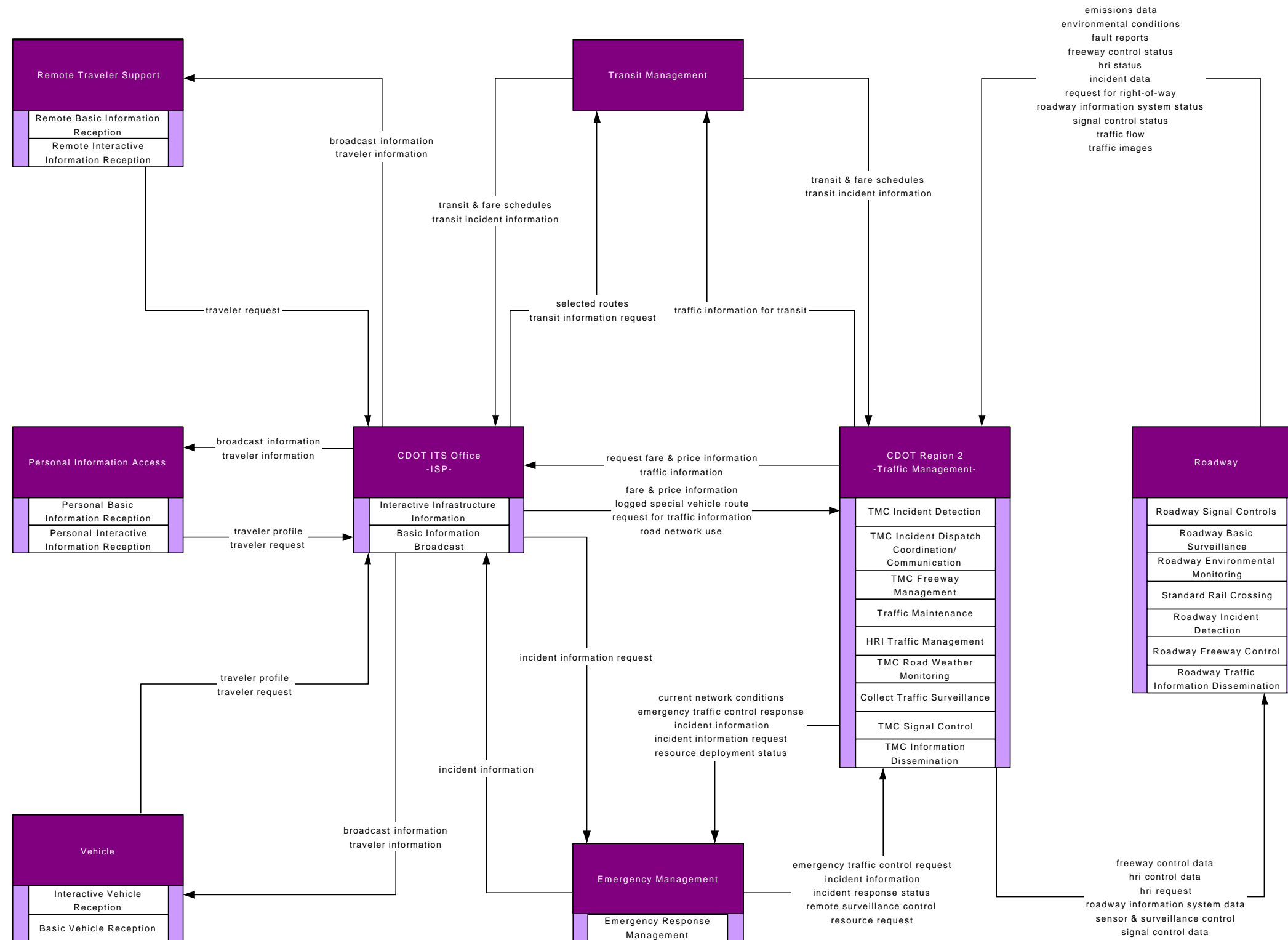
Figure A - 3: CDOT Region 2 ITS Architecture – CDOT Region 2 View
