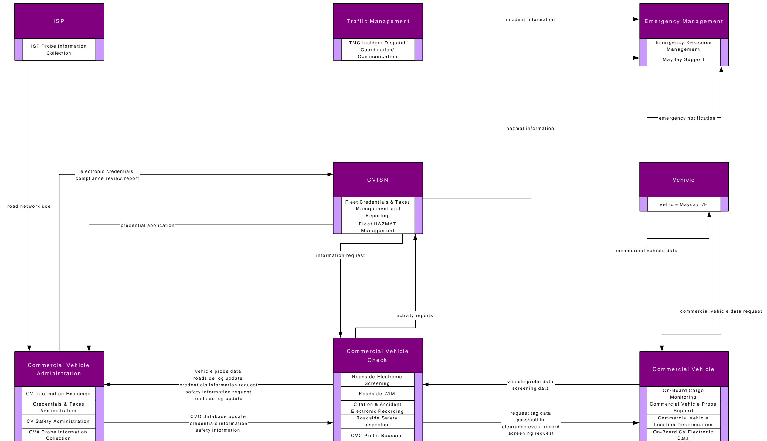
Figure A - 9: CDOT Region 2 ITS Architecture – CVISN View
